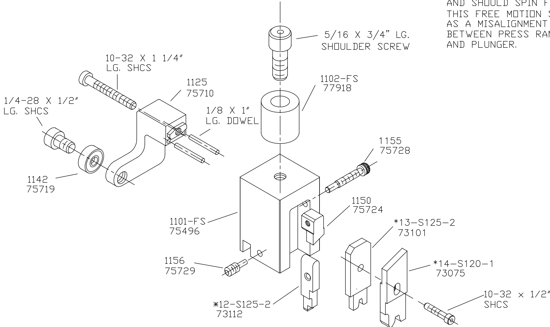
PLUNGER ASSEMBLY SIDE FEED S122N
