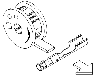
VIEW OF FEED FROM REEL TOWARD APPLICATION (AFTER REWIND)
