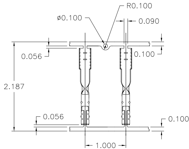
VIEW OF FEED FROM REEL TOWARD APPLICATION (AFTER REWIND)
