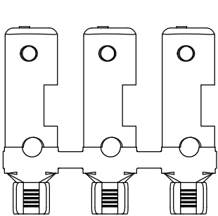
DIRECTION EXITING TOOL, EARS UP, TO THE FRONT
