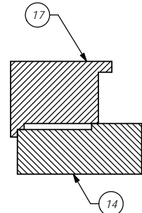
Seat 68017-Rear Guide as such to 68014-Die Plate
