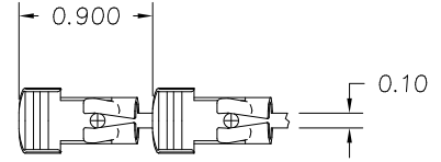
VIEW OF STRIP EXITING FROM TOOL
