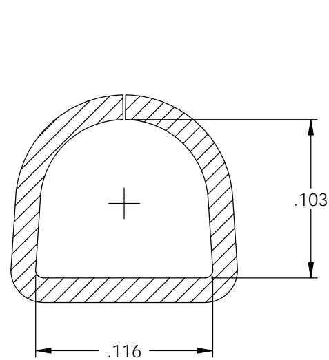
SECTION C-C SCALE 12 : 1
