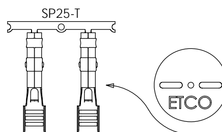
DIRECTION TOWARD APPLICATOR, EARS UP TO THE FRONT, FROM RIGHT
